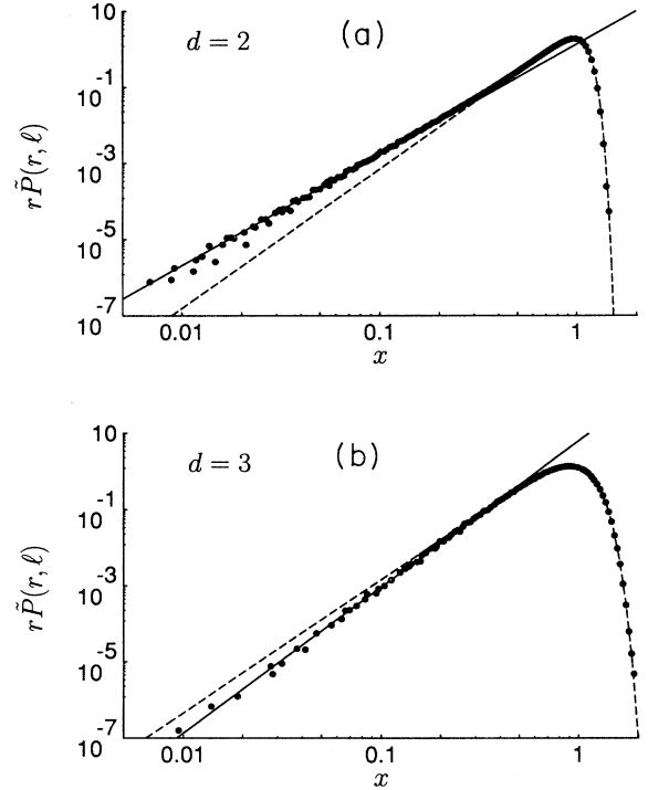
FIG. 1. The structural function for percolation clusters at criticality. Plotted is the function r\tilde{P}(r, \ell) vs x \equiv r/\ell^{\nu} , where \tilde{P}(r, \ell) = r^{d-1}P(r, \ell) , and r\tilde{P}(r, \ell) = x^d f(x) . In d = 2 , \nu \cong 0.88 , and \ell = 250, 500, 750 , and 1000 were used, and averages over 10^6 clusters, grown up to \ell = 10^3 chemical shells, were performed on a square lattice of (2000)^2 sites. In d = 3 , \nu \cong 0.75 , and \ell = 100, 200, 300 , and 500 were used, and averages over 2.5 \times 10^5 clusters, grown up to \ell = 500 chemical shells, were performed on a cubic lattice of (300)^3 sites. None of the clusters touched the boundaries. The lines represent the numerical fits as described in Table I.
